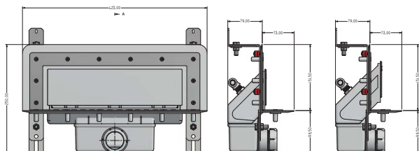
LINNUM WALL - SIFÓN 30mm / 30mm TRAP
