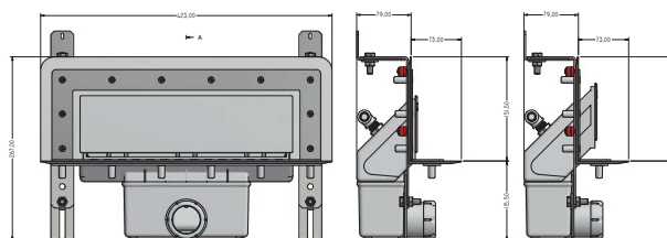
LINNUM WALL - SIFÓN 50mm / 50mm TRAP
